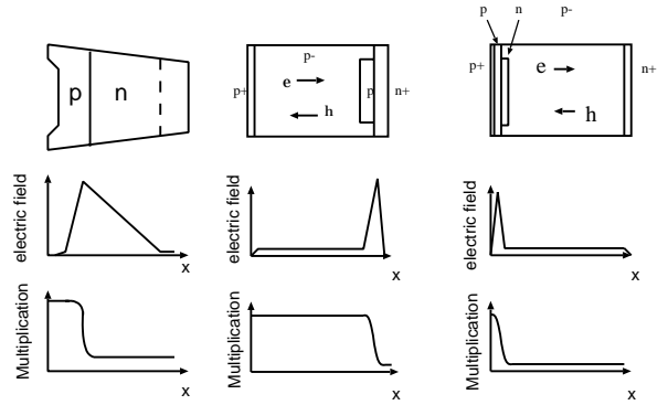
Fig. 1. Internal structures of three different types of APDs. (a) beveled-edge, (b) reach-through, and (c) reverse type (from left to the right). The electric field profiles and the gain profiles in each APDs are also shown in the middle and bottom panels.
