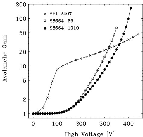
Fig. 2. Gain variations of Hamamatsu APDs measured at room temperature ( +20^\circ\text{C} ).
