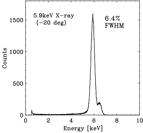
Fig. 3. Energy spectrum of 5.9 keV X-rays at -20^{\circ}\text{C} .
